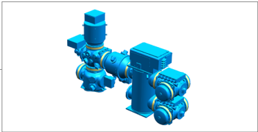
Developed 72.5kV 31.5kA SF 6 -Free GIS
